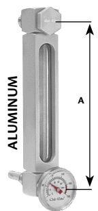
Thermometer AD862
